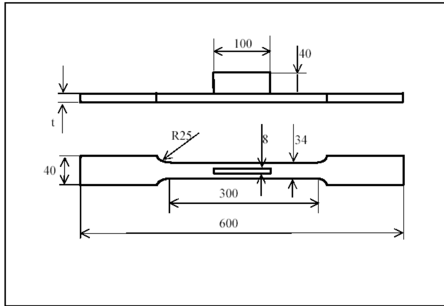
Figure 4. Geometry of the longitudinal non-load carrying welded specimen ( t=5\text{mm} or 8\text{mm} ).
